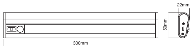
PG Linear LED Mobile USB 300mm MiPRC
