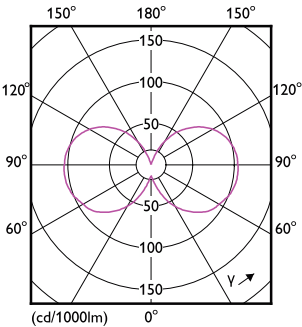
Light Distribution Diagram - MAS VLE LEDBulbD3.4-40W E27 940 A60CL G
