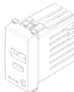
Vista 3D
